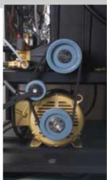
The Tru-Tite belt tensioning system minimizes wear and tear on the belt.
